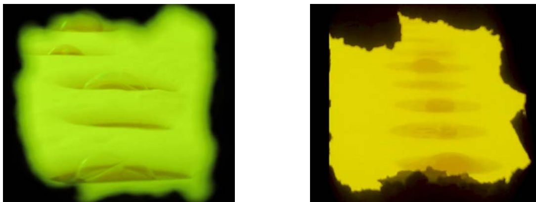
Figure 13: Clearing of foam around bubblers with HR x burners at 290 TPD flint container glass melting furnace.
