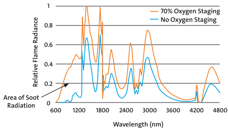
Figure 1: Graph showing radiation spectra for oxy-fuel flames without oxygen staging and with oxygen 70% staging.
